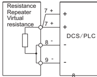
3-wire (+, -, -)
