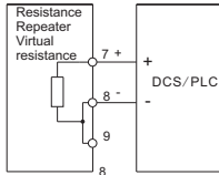
3-wire (+, +, -)
