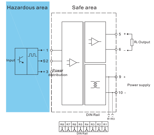
Single input, single output
